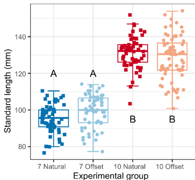
Fig. 3. Standard length of individual age-1 herring reared under different light (natural and offset) and temperature (7 and 10°C) regimes. Horizontal lines represent medians, boxes represent the interquartile range (IQR), and whiskers represent the lowest and highest observations within 1.5× IQR. Individual points indicate raw data. Compact letter displays of all pairwise comparisons based on the 2-way ANOVA (Table S1) are provided to demonstrate statistical differentiation
